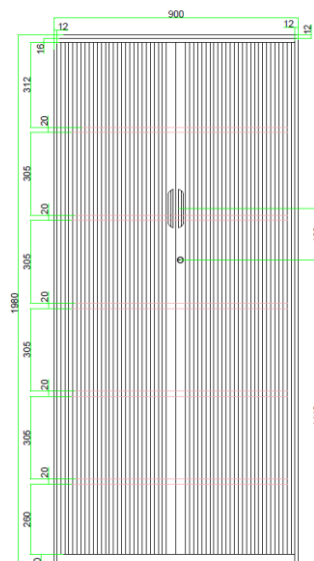
DT-H1980-90-B/W 5 levels - Adjustable Recommended spacing: 1 st FFL : 260mm 1-4 th FFL : 305mm 5 th FFL : 312mm Shelves : 5 included
